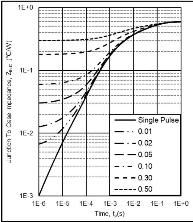
Figure 21. Transient thermal impedance (Junction - Case)
